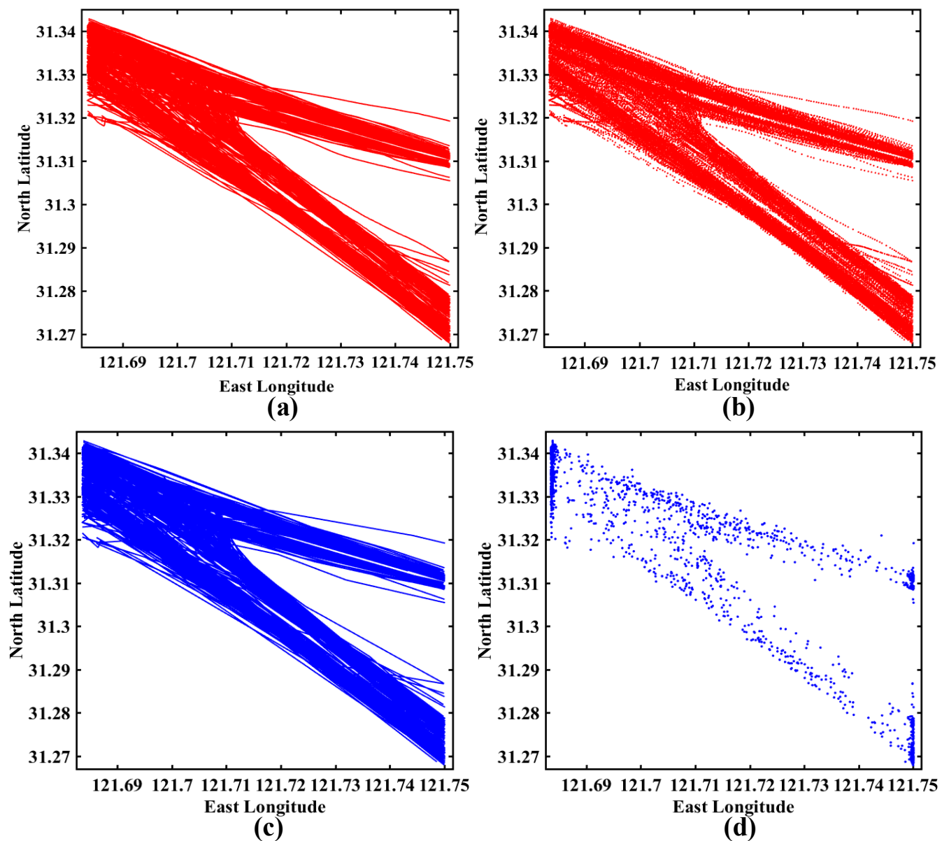
FIGURE 4. The original and compressed trajectories of inland waterway: (a) the original vessel trajectories; (b) the original point data (c) the trajectories after compression by ADP; (d) the point data after compression by ADP.
