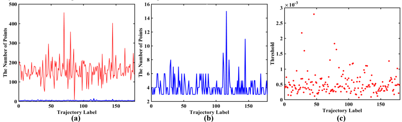
FIGURE 9. Visualization of the number of points and the threshold of down-bound trajectories: (a) the number of points before and after compression; (b) the number of points after compression; (c) the threshold of each trajectory.
