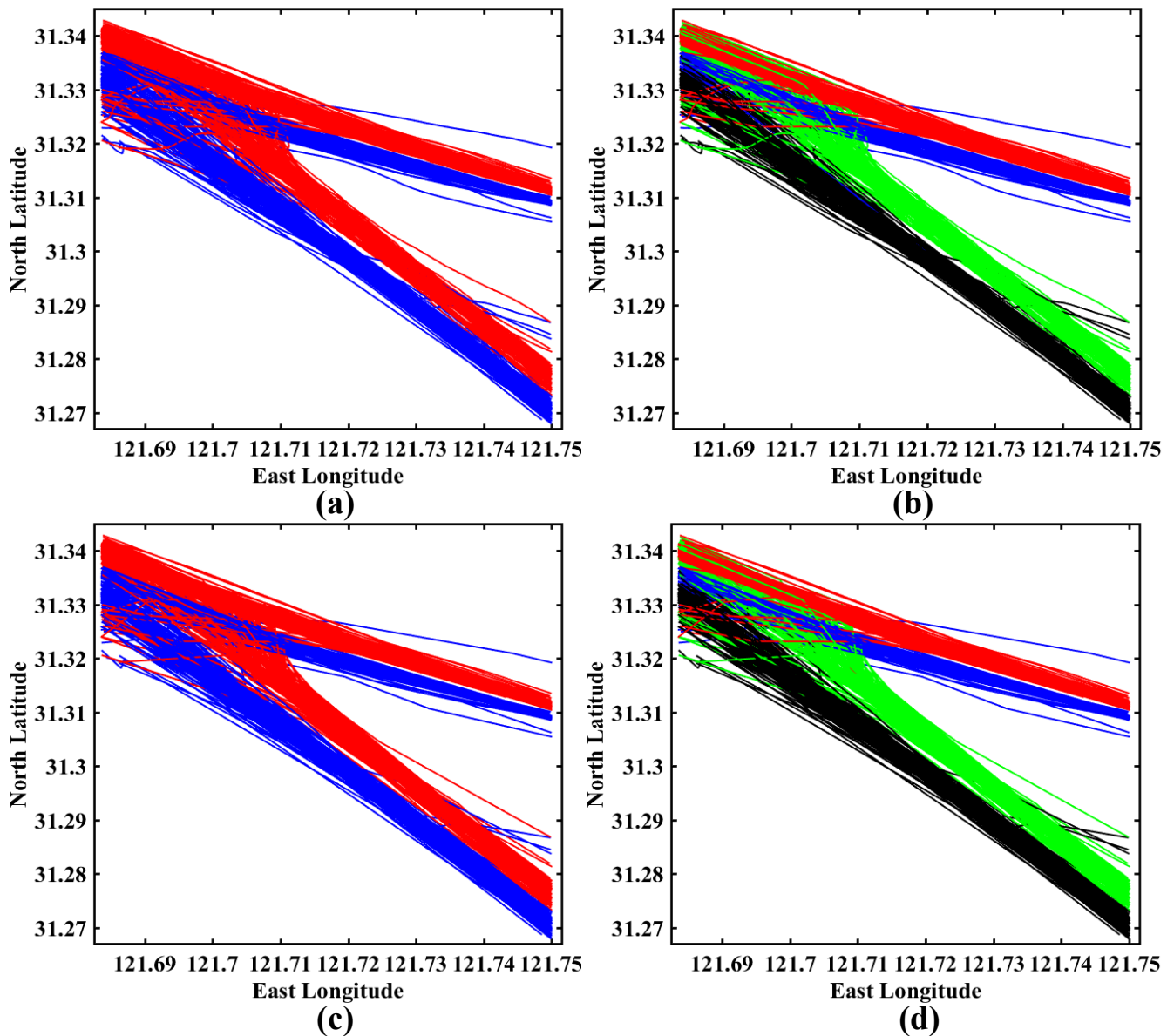
FIGURE 13. The classification results of data set in the inland waterway: (a) visualization of the original data set; (b) the classification results of the original data set; (c) visualization of the data set with ADP; (d) the classification results of the compressed data set.
