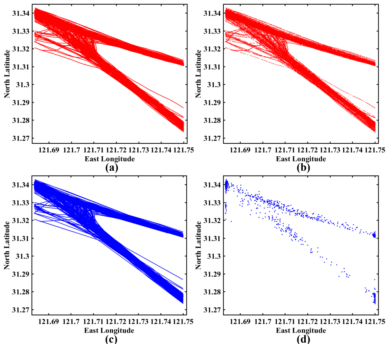
FIGURE 6. The original and compressed trajectories of up-bound vessels: (a) the original vessel trajectories; (b) the original point data (c) the compressed trajectories by ADP; (d) the point data after compression by ADP.
