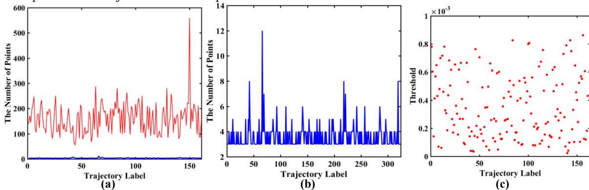
FIGURE 11. Visualization of the number of points and the threshold: (a) the number of points before and after compression; (b) the number of points
