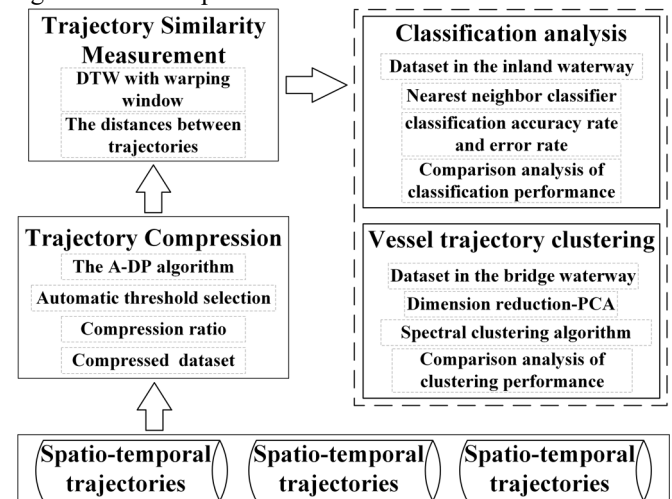
FIGURE 2. The flowchart of our proposed method
