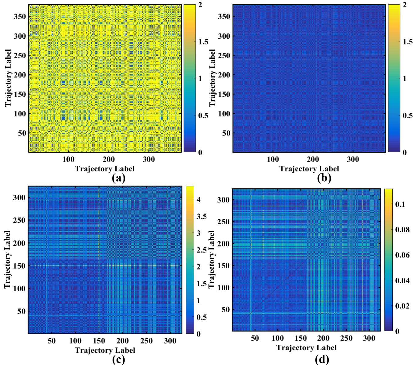
FIGURE 12. Visualization of the distance matrix: (a) 2D image visualization of the 380 \times 380 distance matrix before trajectory compression; (b) 2D image visualization of the 380 \times 380 distance matrix after trajectory compression; (c) 2D image visualization of the 324 \times 324 distance matrix before trajectory compression; (d) 2D image visualization of the 324 \times 324 distance matrix after trajectory compression.
