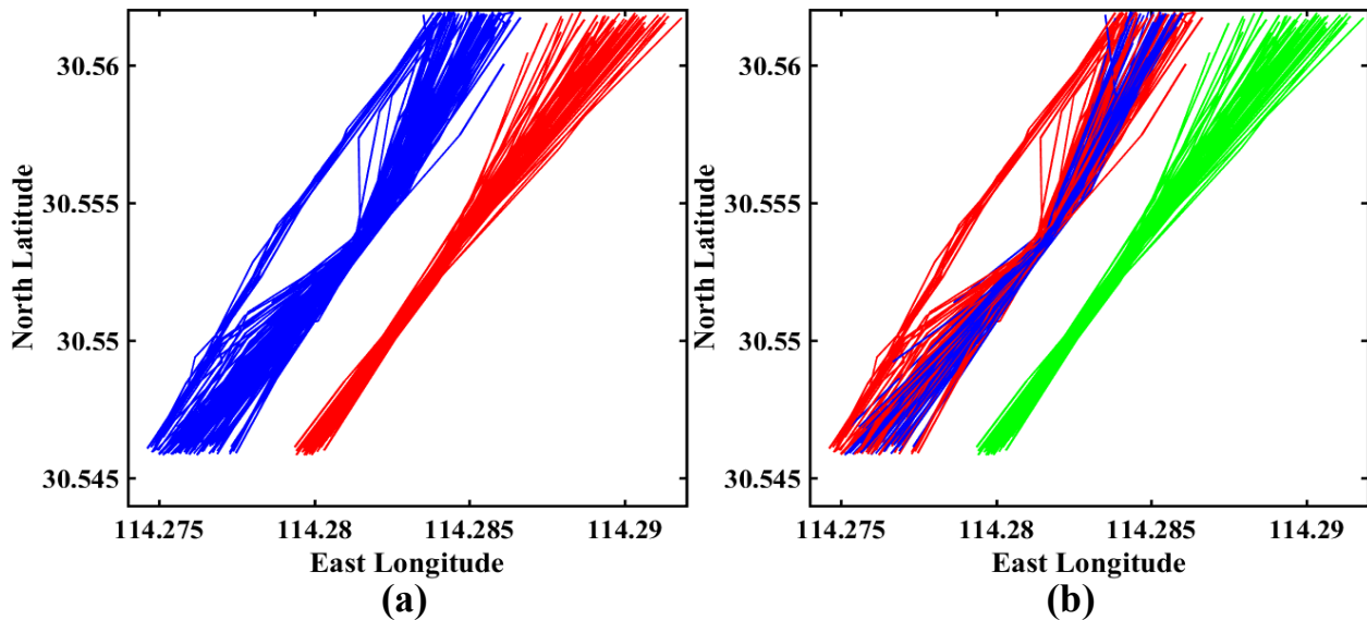
FIGURE 15. The clustering results of the bridge area waterway data set: (a) the clustering results based on spectral clustering (k=2); (b) the clustering results based on spectral clustering (k=3).
