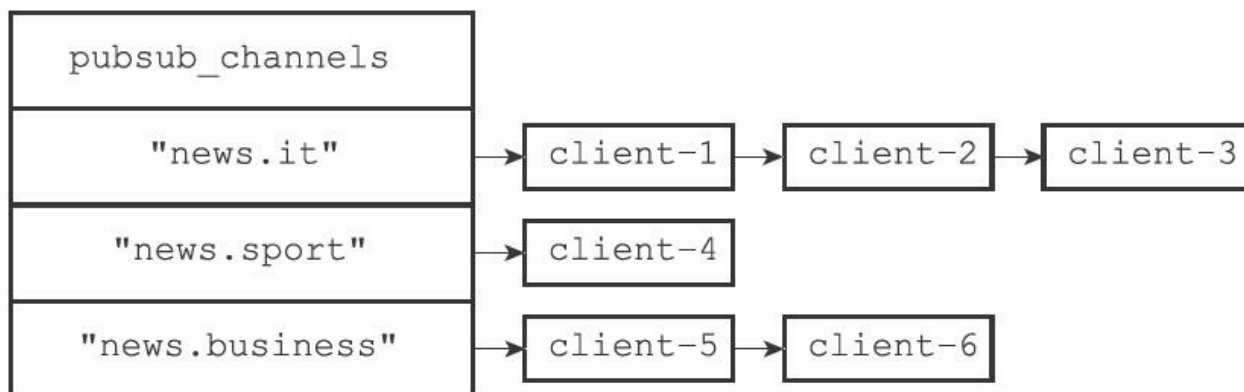
图18-16 pubsub_channels字典
