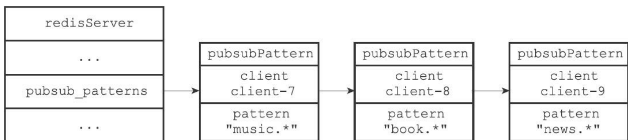
图18-17 psubsub_patterns链表
