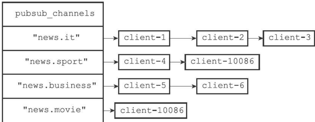
图18-19 pubsub_channels字典
