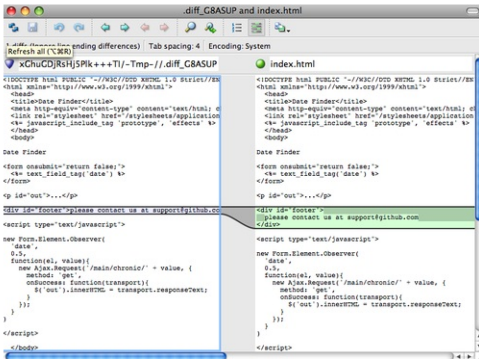
Figure 8-1. P4Merge.
